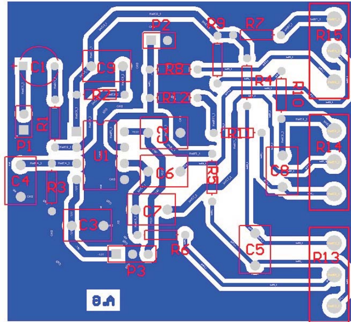
Components Placement - Top Side View
