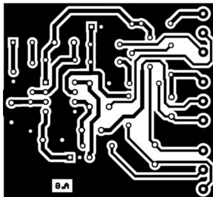
PCB - Layout in 1:1 scale
