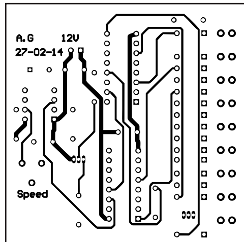
Top-side (Components side)
