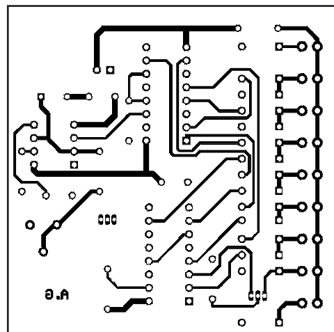
Bottom-side
