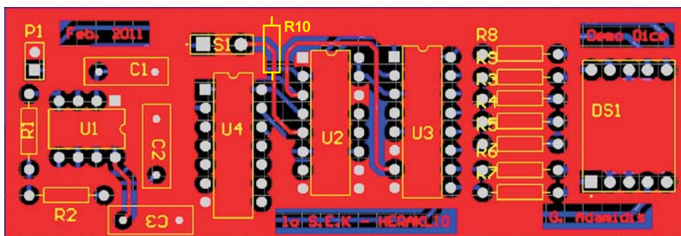
Assembly details - Top View
