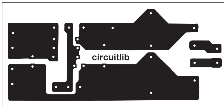
PCB Layout in 1:1 scale - Copper Side
