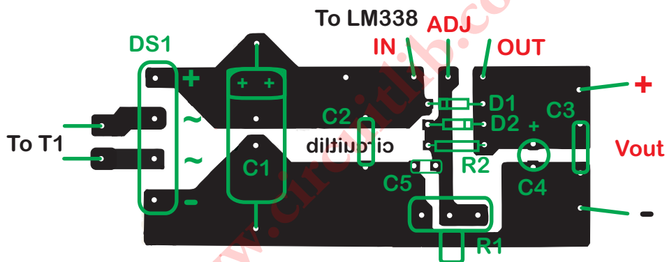
Components Placement guide - Top View
