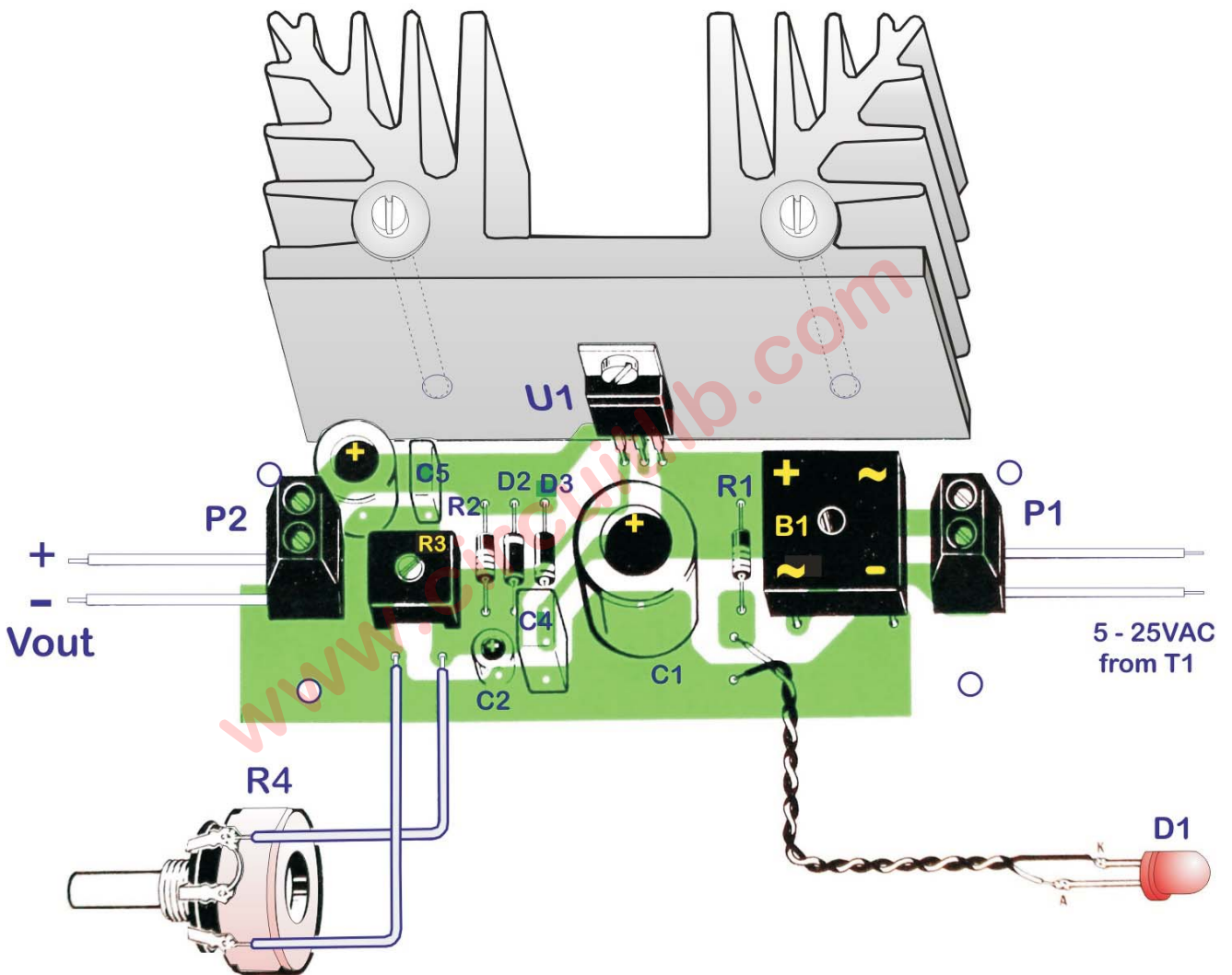
Assembly details - Components side
