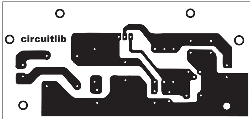
PCB Layout / 1:1 scale -Copper Side
