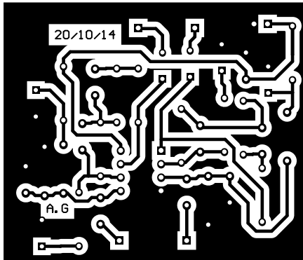
Printed Circuit Board - 1:1 scale
