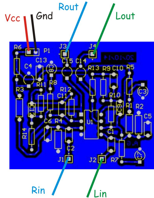
Components placement - Top view
