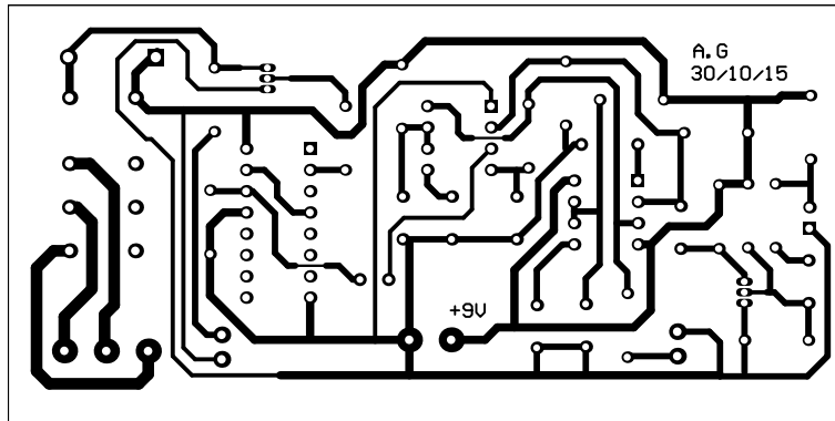
Clap Switch PCB in 1:1
