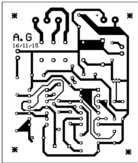
Simple Electronic Lock Printed Circuit Board in 1:1 Copper Side
