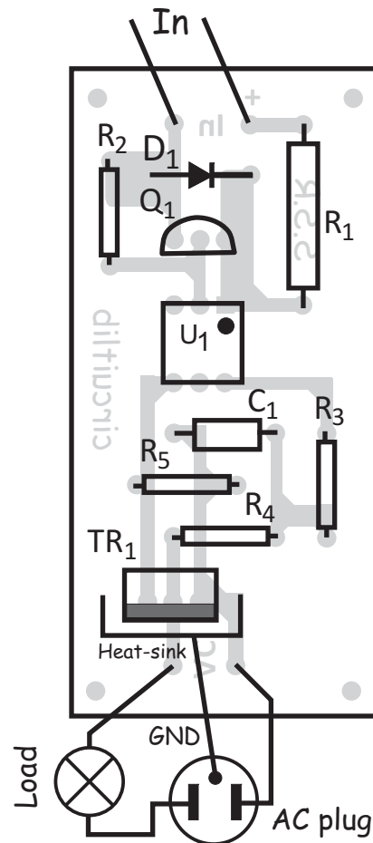
Components placement
