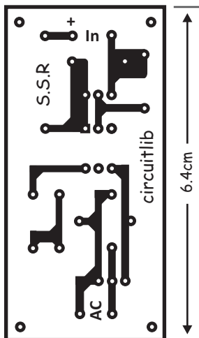
PCB layout
