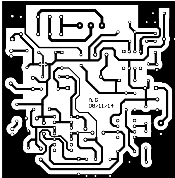
Printed Circuit Board in 1:1 scale
