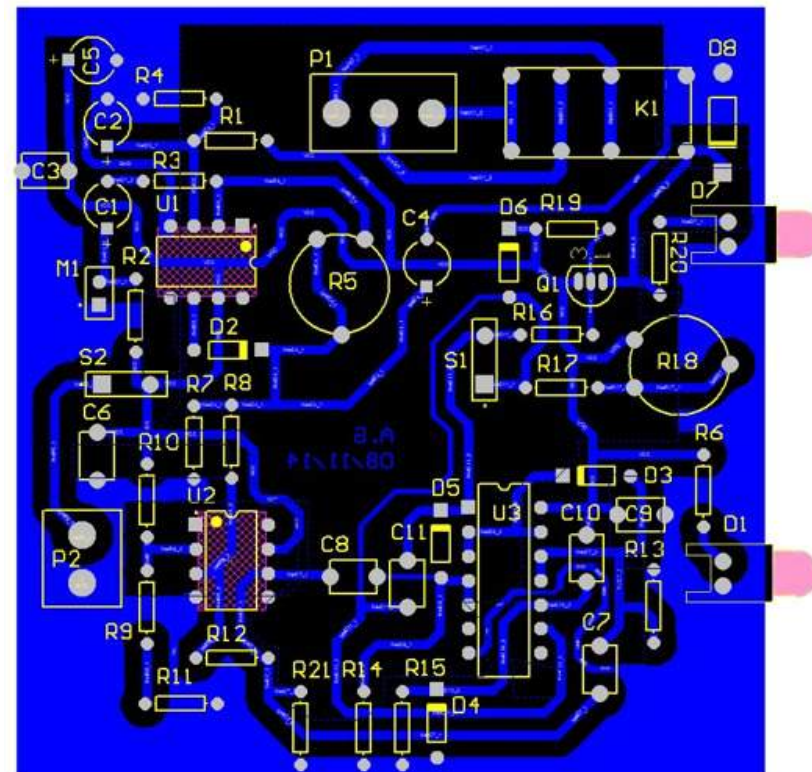
Components placement guide
