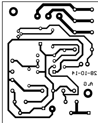
Printed Circuit Board in 1:1 scale
