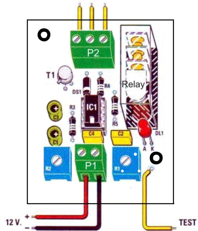
Components Placement - Top view
