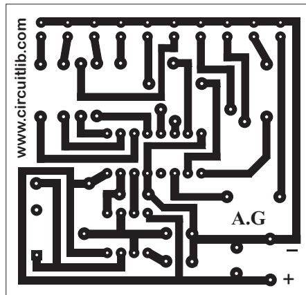
PCB - Bottom view
