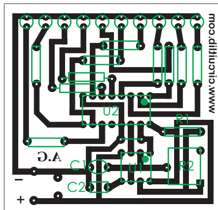
Assembly details -Top view
