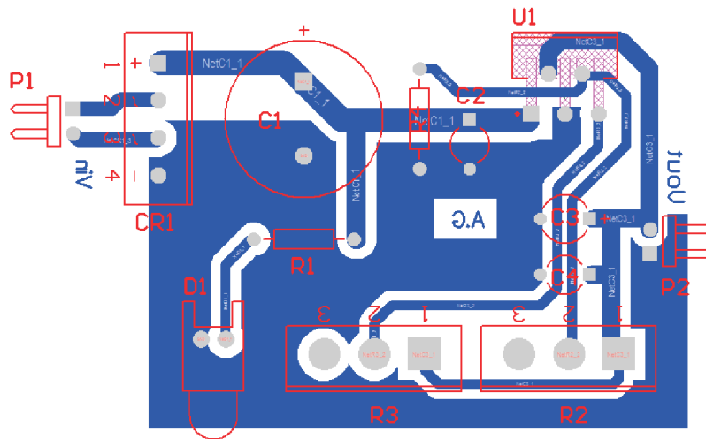
Components Placement - Components side view
